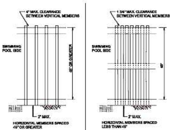
Figure 3109.4.1.3 PRIVATE SWIMMING POOL BARRIER CONSTRUCTION
