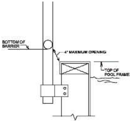
Figure 3109.4.1 OPENING LIMITATIONS
